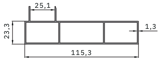
Çift Cam Alt Kasa Profili Double Glazing Bottom Frame Profile : 1.206 kg/m
